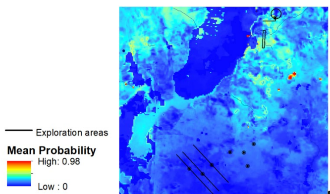
Figure 55: Mean probability of presence of Gouldian Finch within the exploration areas (Young et al., 2022)
