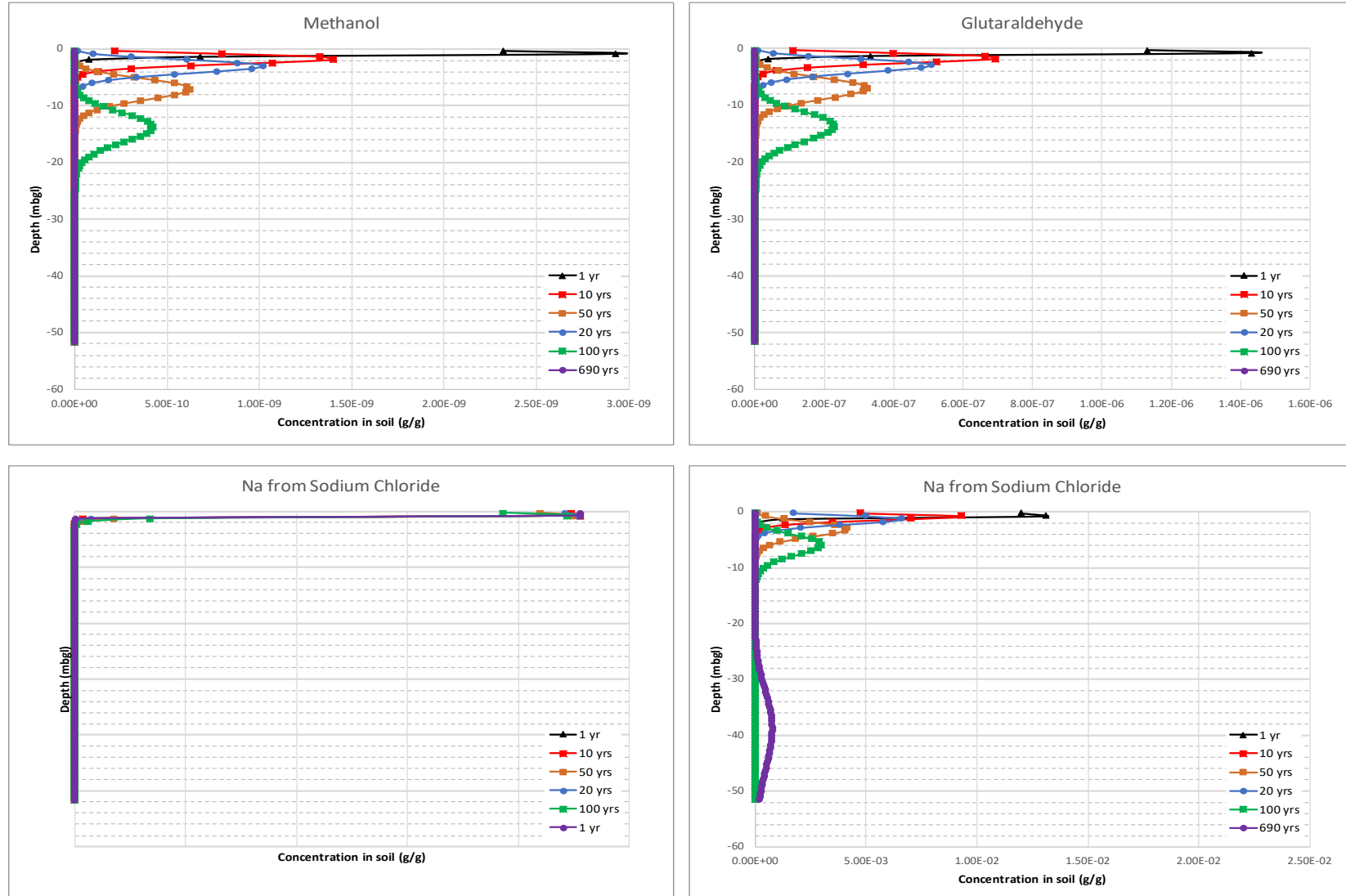
Figure 4-2 VLEACH Results (Note: Bottom left Na assumes a distribution coefficient 2 orders of magnitude higher then bottom right results.)
