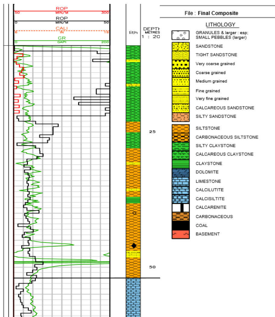
Figure 2-2 Shallow Lithology from well "Tanumbirini-1"
