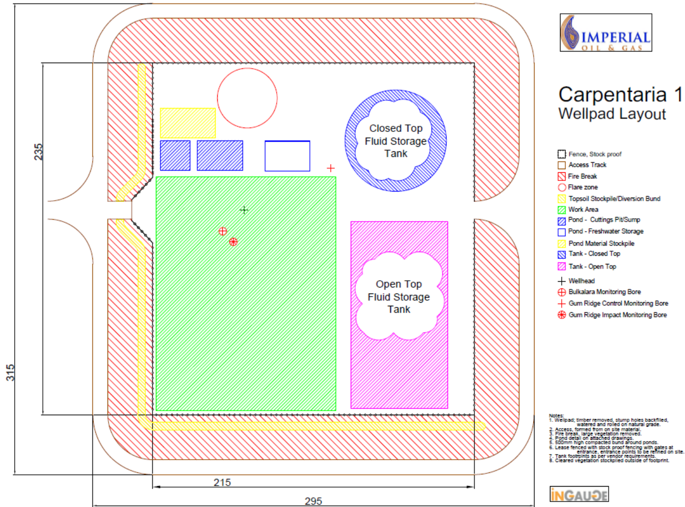
Figure 2: Wellpad Layout
