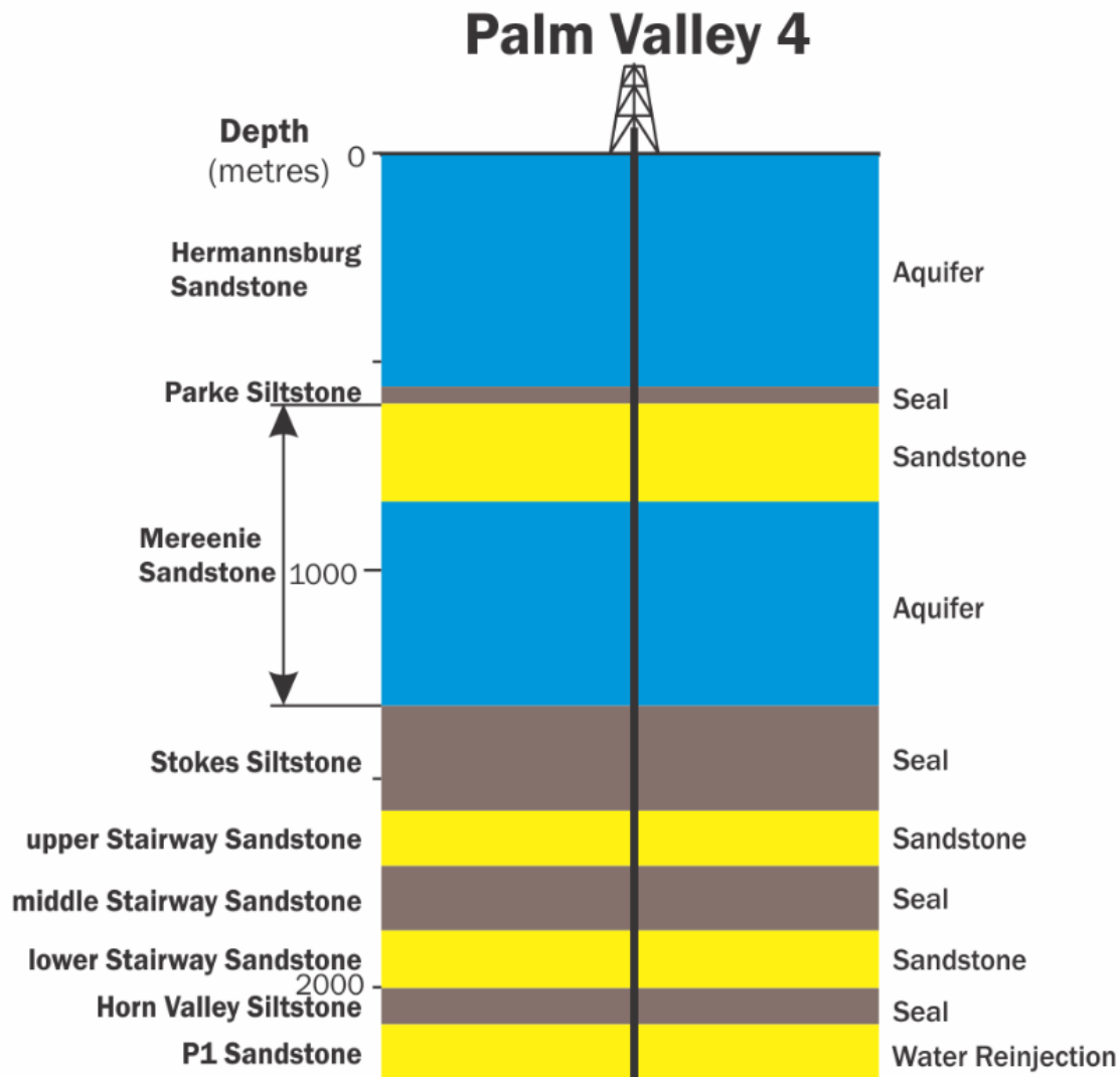
Figure 6-8 Palm Valley 4 cross section of stratigraphy
