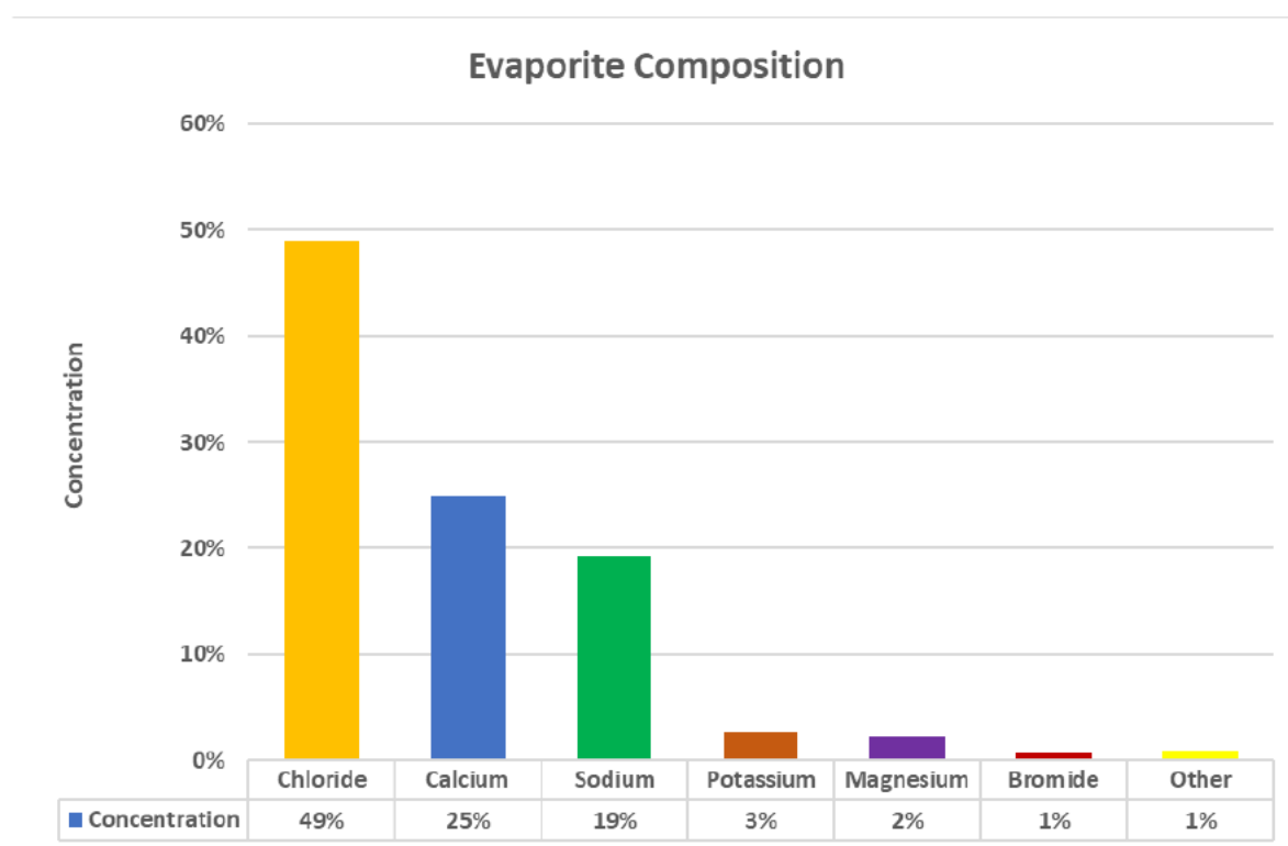
Figure 13: Evaporite composition – PV-09
