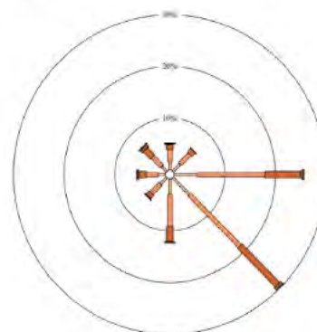
Average rainfall
