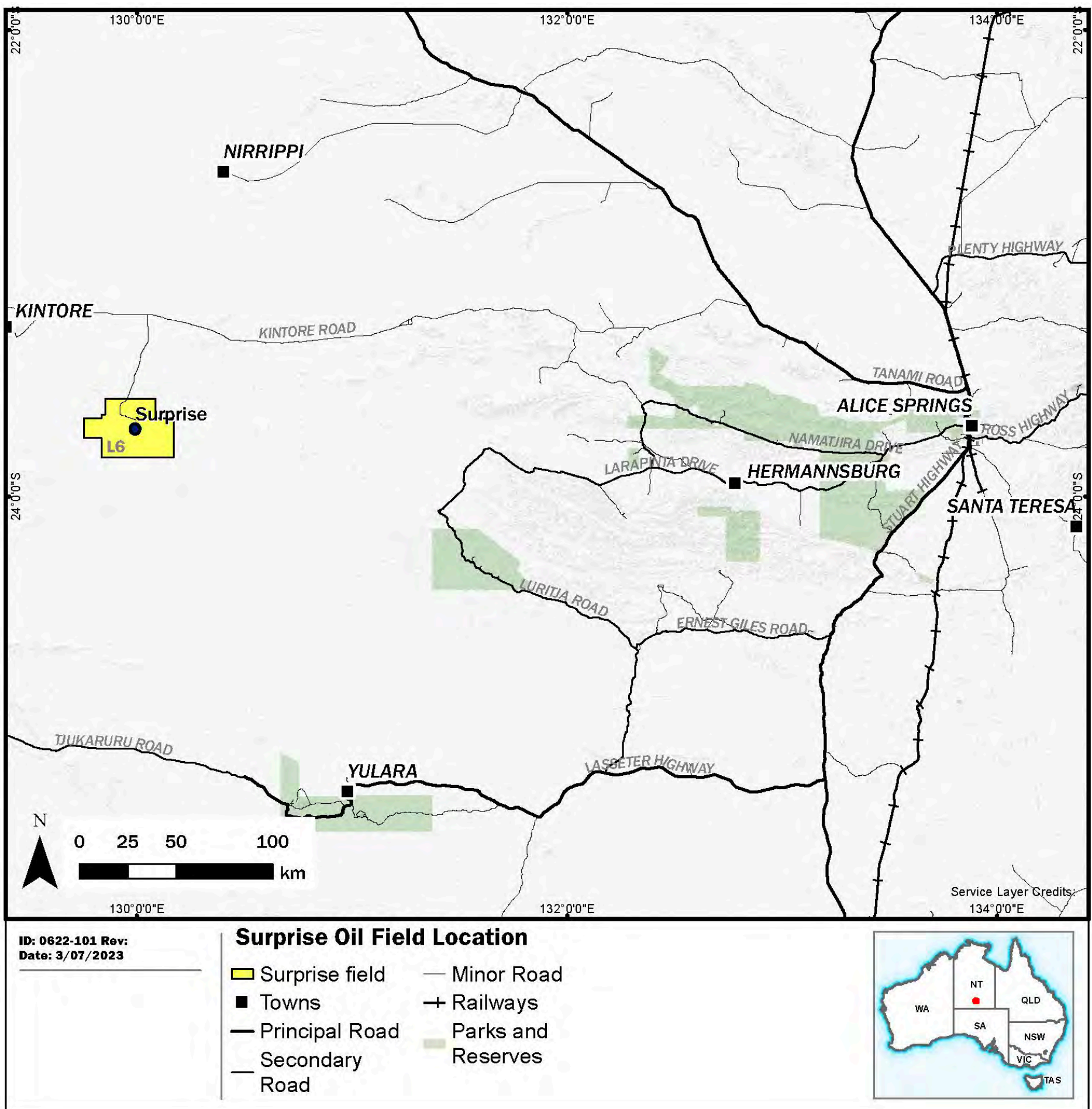
Figure 4: Location Map of the SOF
