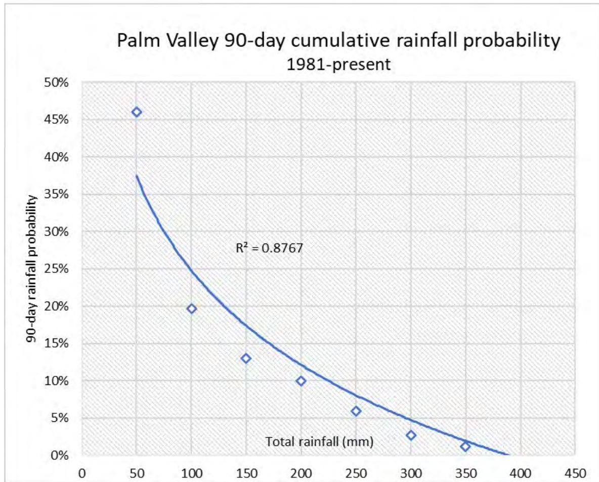
Figure 12: 90-day cumulative rainfall event probability PVGF (BOM 15633)
