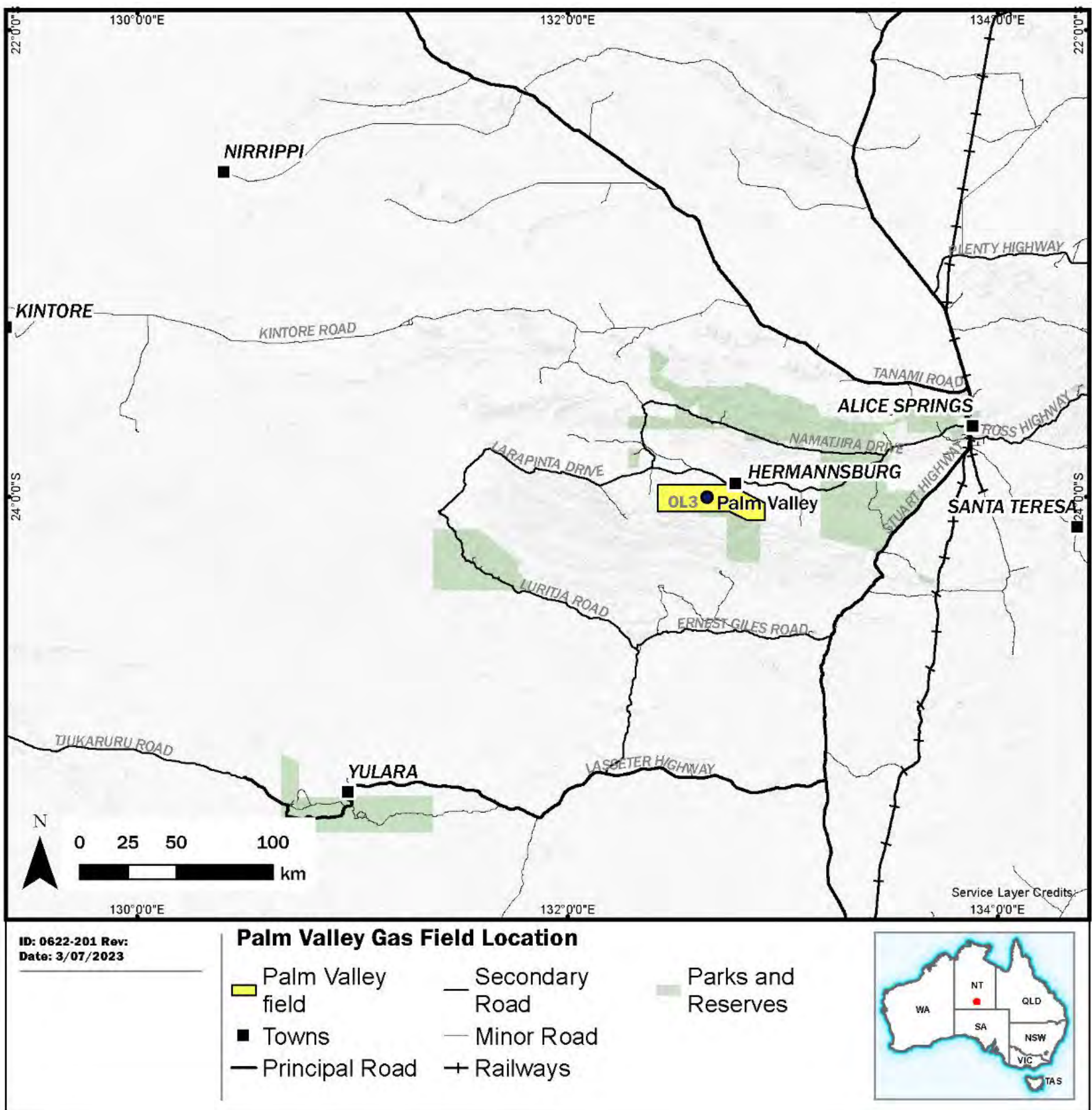
Figure 2: Location Map of the PVGF
