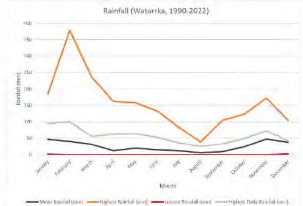
Average rainfall
