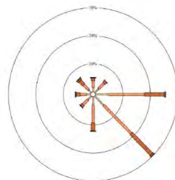
Average rainfall
