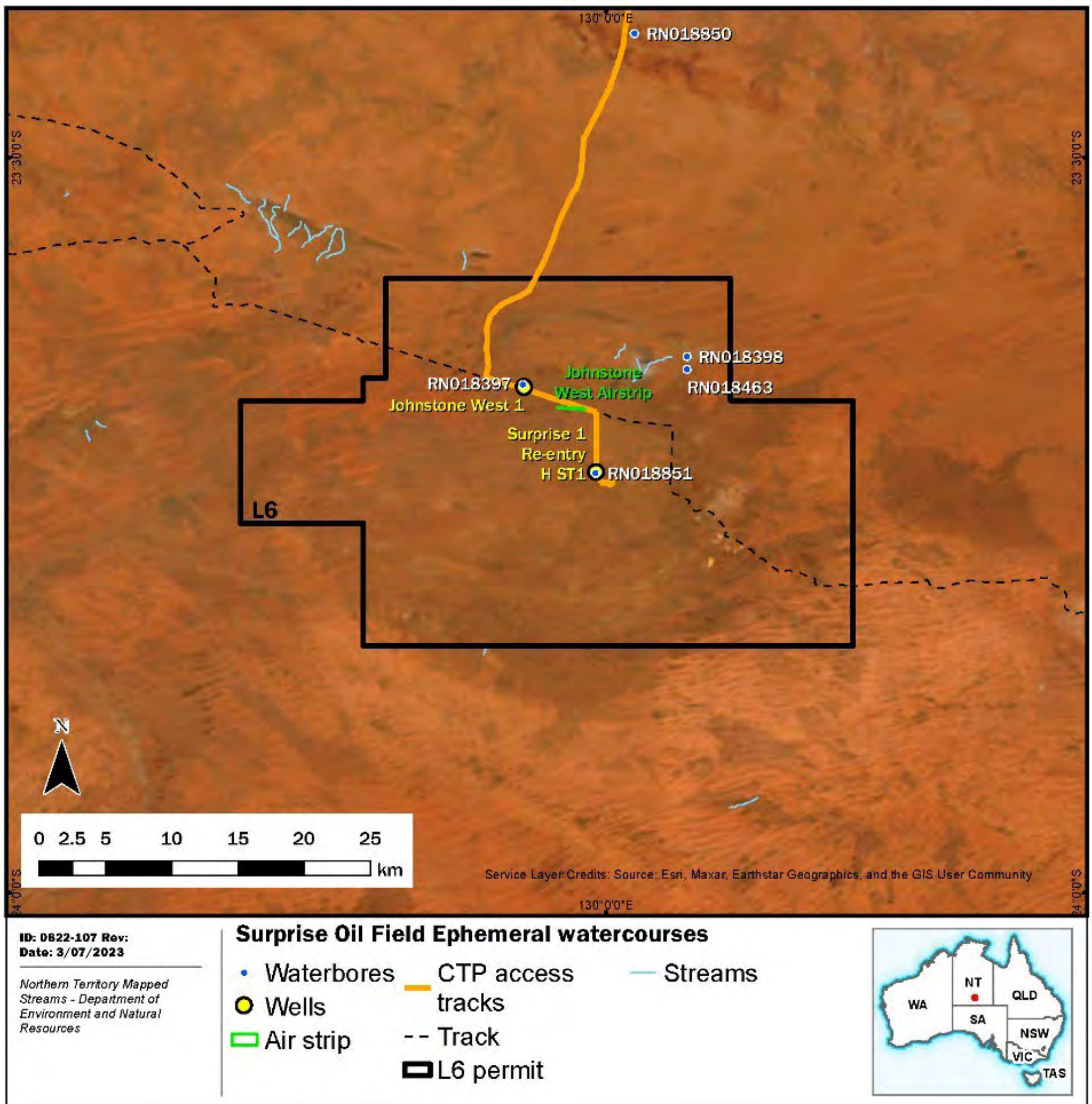
Figure 21: Ephemeral water courses SOF
