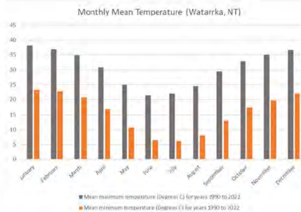
Average temperatures
