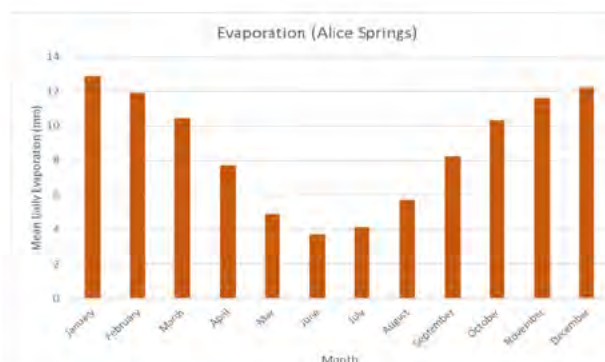
Average evaporation rates
