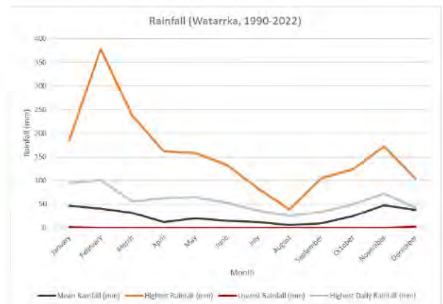
Average rainfall
