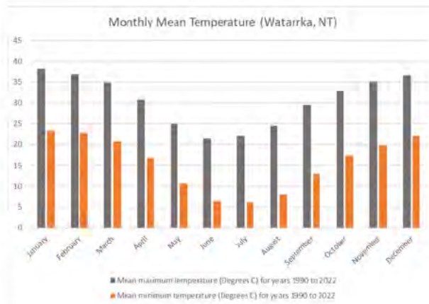
Average temperatures
