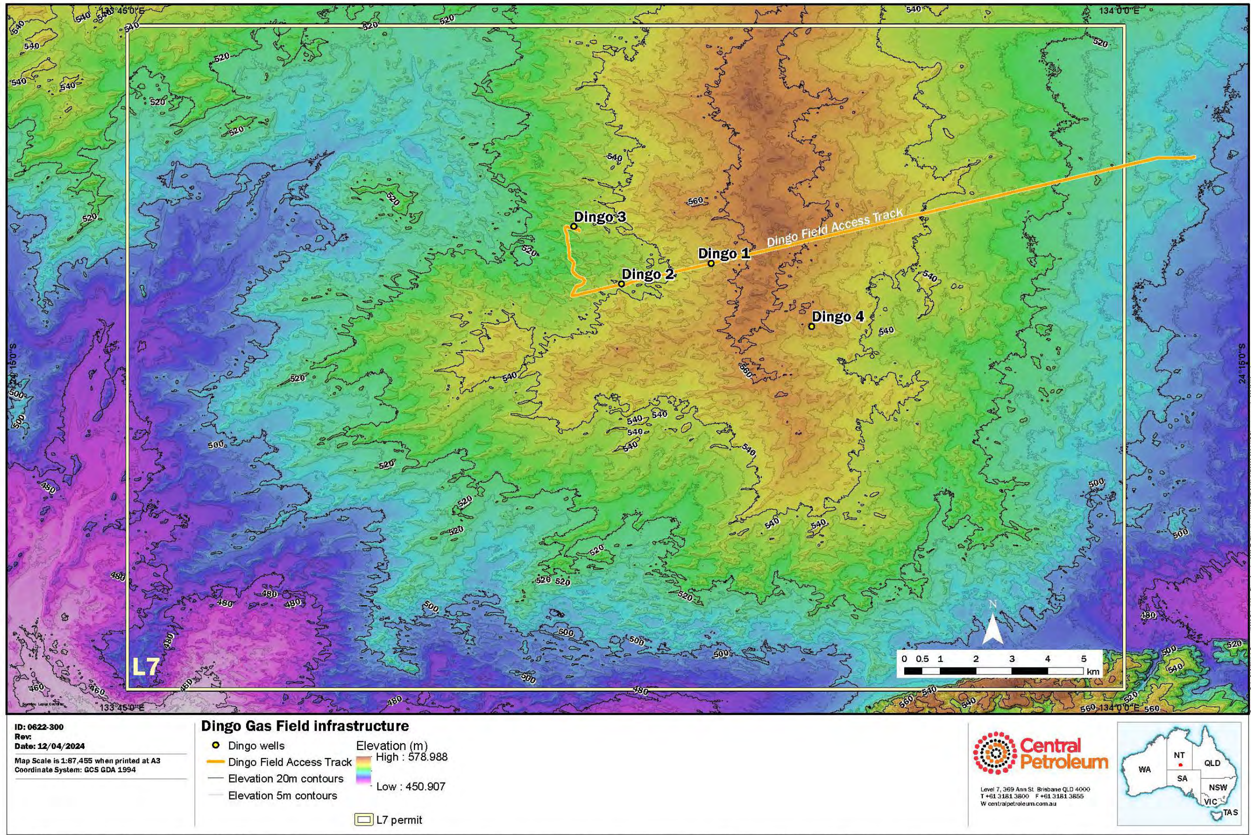
Figure 17: Topographic map of DGF well pads and infrastructure
