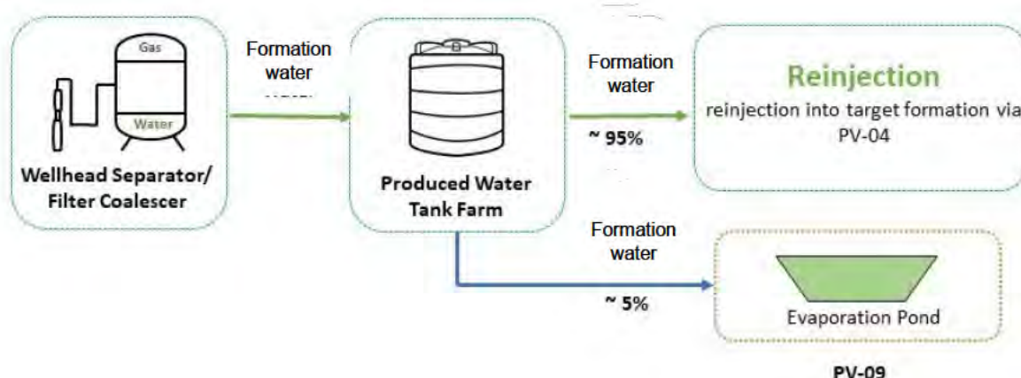
Figure 9: PVGF produced formation wastewater process
