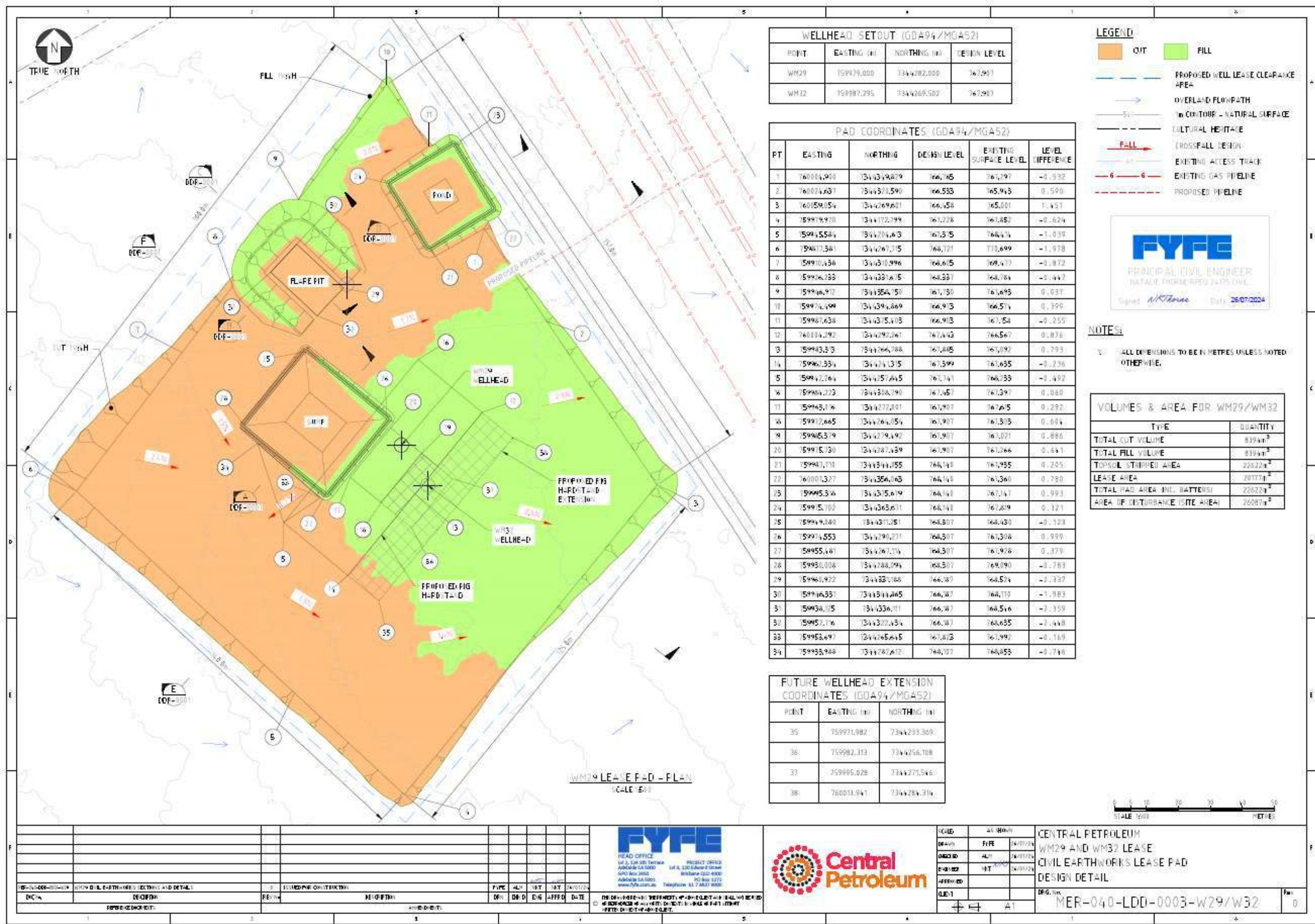
Figure 11: WM32 Option A indicative Civil drawing
