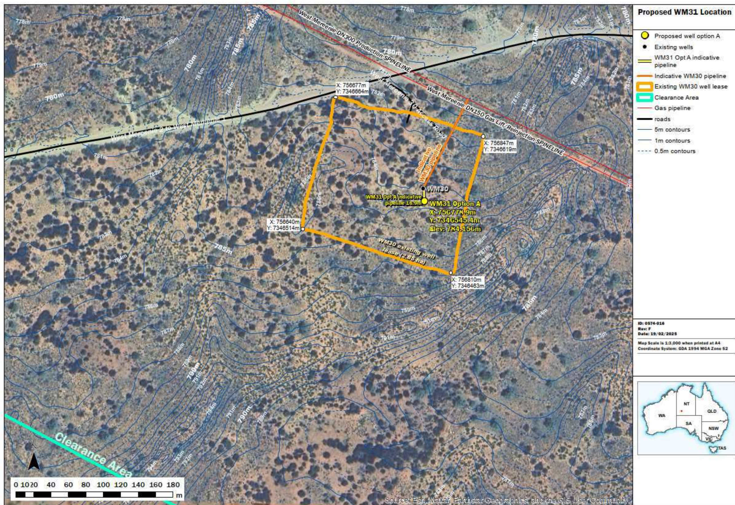
Figure 4: Location of WM31 Option A well site – well site, access track, flowline corridor
