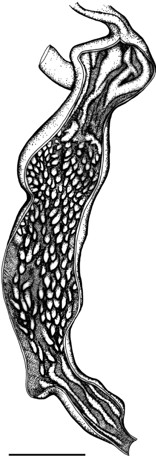
Fig. 13. Detail of penis of Torresitrachia alenae sp. nov. Penial wall opened along its length to reveal detail of internal ornamentation. Scale 1.5 mm. See Fig. 4 for labelling of structures.
