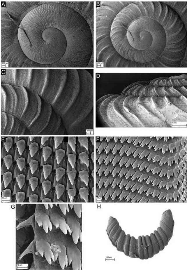
Figure 5. SEM photographs of shells, radula and jaws of Torresitrachia wallacei sp. nov., paratypes AM C.462998: A , Close-up of protoconch (scale 100 \mu m); B , Apical portion of shell with first whorls viewed from above (scale 200 \mu m); C , Sculpture on second to fourth whorls viewed from above (scale 200 \mu m); D , Lateral view of shell (scale 1 mm); E , Close-up of central (white arrow) and inner lateral teeth (scale 10 \mu m); F , Inner and middle marginal teeth (scale 10 \mu m); G , Close-up of middle marginal teeth (scale 10 \mu m); H , Jaw (scale 100 \mu m).
