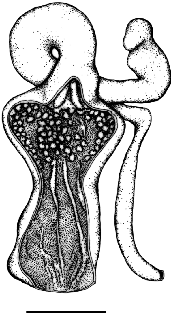
Fig. 10. Detail of penis of Torresitrachia cuttacutta sp. nov. Penial wall opened distally to reveal detail of internal ornamentation. Scale 0.5 mm. See Fig. 4 for labelling of structures.
