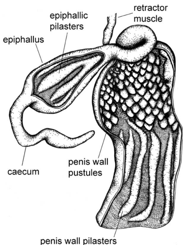
Fig. 4. Detail of penis of Torresitrachia darwini sp. nov. Penial wall opened proximally and distally to reveal detail of internal ornamentation. Scale 0.5 mm.
