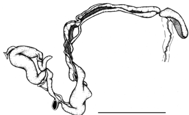
Figure 6. Genital system of Torresitrachia wallacei sp. nov. Scale 5 mm. See Fig. 3 for labelling of organs.
