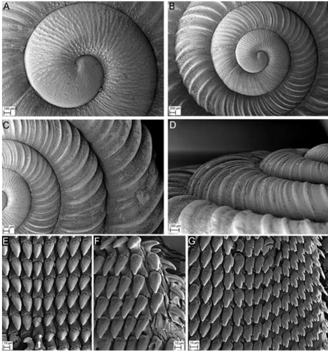
Fig. 2. SEM photographs of shells and radula of Torresitrachia darwini sp. nov., paratypes AM C.463000: A , Close-up of protoconch (scale 100 µm); B , Apical portion of shell with first whorls viewed from above (scale 200 µm); C , Sculpture across all whorls of shell viewed from above (scale 200 µm); D , Lateral view of shell (scale 200 µm); E , Central (white arrow) and inner lateral teeth (scale 10 µm); F , Close-up of lateral teeth (scale 10 µm); G , Outer lateral and inner marginal teeth (scale 10 µm).
