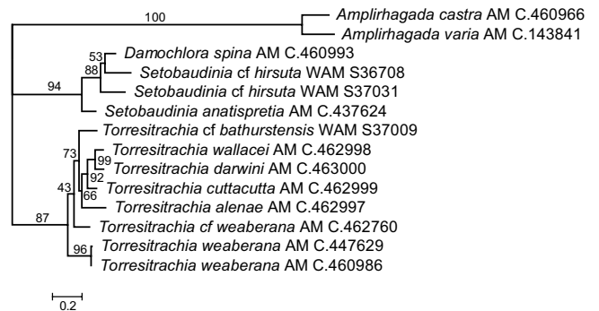
Fig. 15. Maximum Likelihood tree based on analysis of a partial fragment of the mitochondrial 16S rRNA gene (length of unaligned sequences approx. 750 bp) for a general time-reversible model of sequence evolution with gamma-distributed rate heterogeneity (GTR+I+ \Gamma ). Numbers on branches indicate nodal support by expected likelihood weights to all rearrangements of tree topology (WLW-LR; Strimmer and Rambaut 2002).
