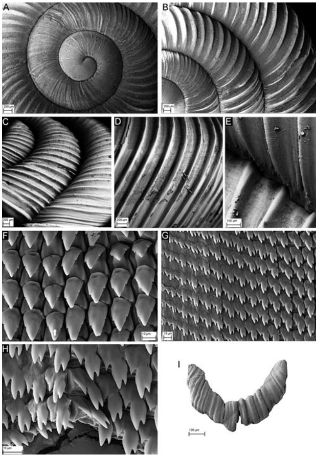
Figure 8. SEM photographs of shells, radula and jaws of Torresitrachia cuttacutta sp. nov., paratypes AM C.462999: A , Apical portion of shell with first whorls viewed from above (scale 200 µm); B , Surface across all whorls of shell as viewed from above (scale 200 µm); C , Surface of third to fifth whorls viewed obliquely from above (scale 100 µm); D , Close-up of sculpture on body whorl (scale 200 µm); E , Details of sculpture at suture between body and penultimate whorl; F , Close-up of central (white arrow) and inner lateral teeth (scale 10 µm); G , inner and middle marginal teeth (scale 10 µm); H , Close-up of middle marginal teeth (scale 10 µm); I , Jaw (scale 100 µm).
