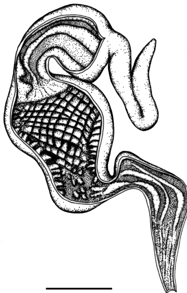
Fig. 7. Detail of penis of Torresitrachia wallacei sp. nov. Penial wall opened along its length to reveal detail of internal ornamentation. Scale 1 mm. See Fig. 4 for labelling of structures.
